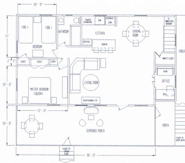
MAIN FLOOR
